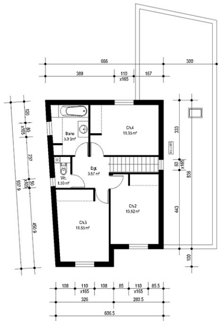
PLAN ETAGE 1/100 eme
