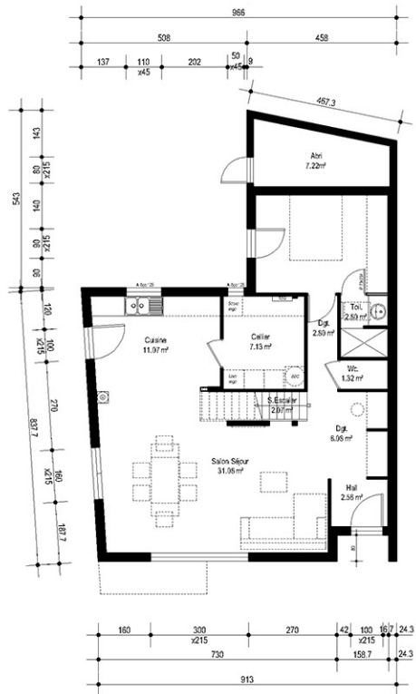
PLAN RDC 1/100 eme
